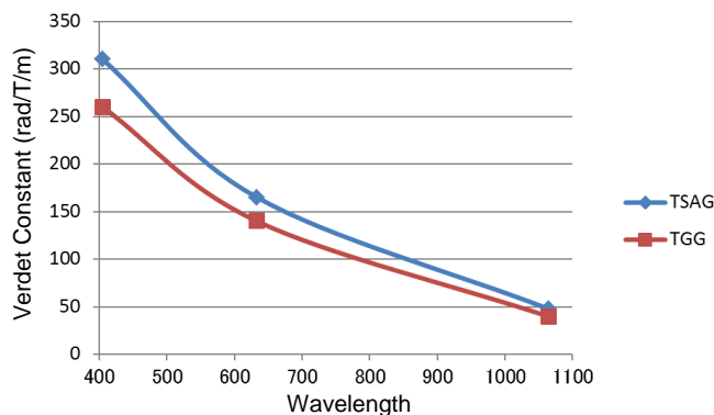
Verdet Constant vs. Wavelength at 400-1064 nm
