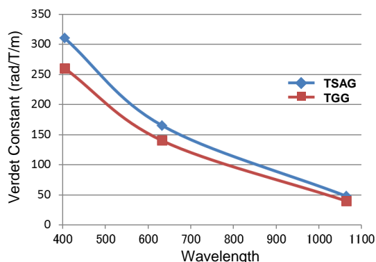
Verdet Constant vs. Wavelength at 400-1064 nm
